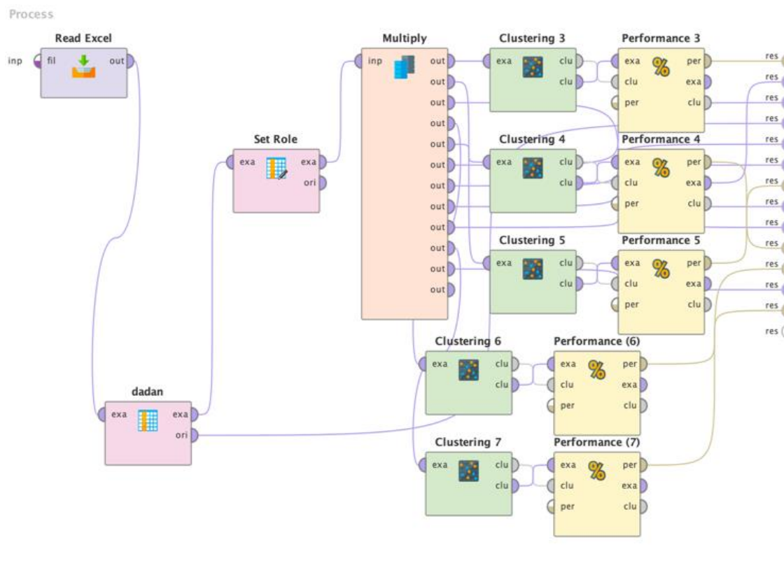
Figure 4. Clustering process
